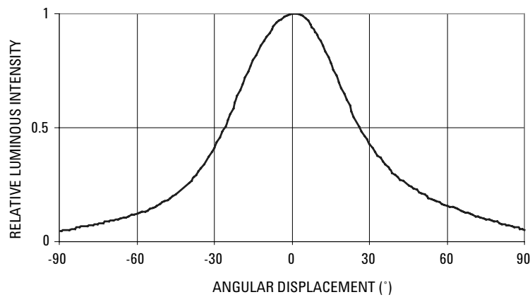
Figure 6. Spatial Radiation Pattern for CW4x
